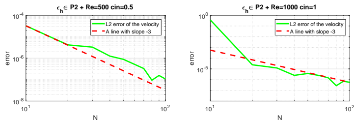
Figure 4: L^2 error for the velocity using \varepsilon_h \in \mathbb{P}_2 . (Left): (Re, c_{in}) = (500, 0.5) , (Right): (Re, c_{in}) = (1000, 1) .
